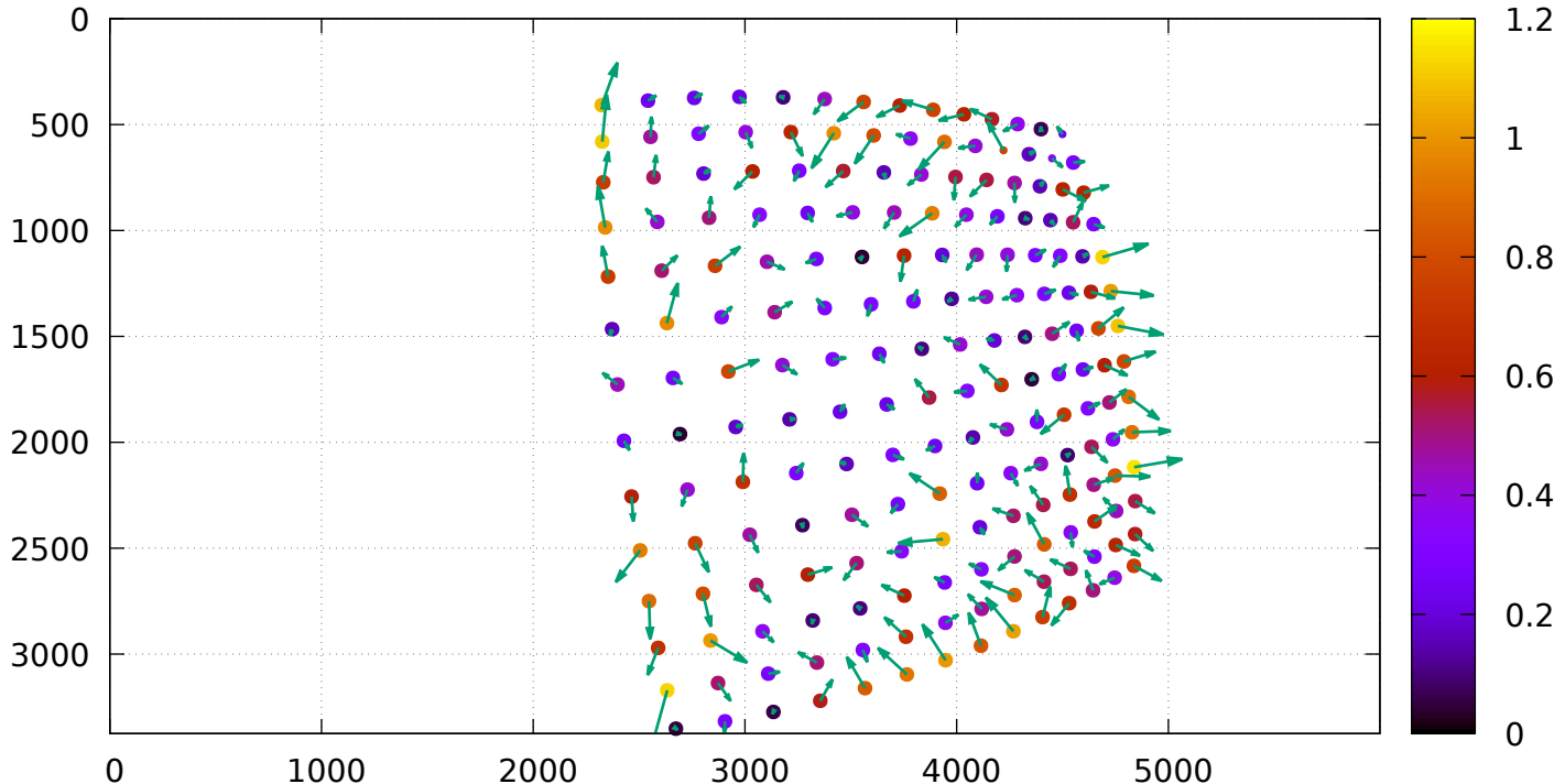
Residuals from a dynamic chessboard shape error
