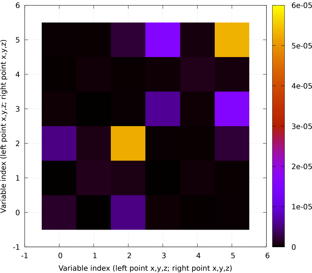
Abs(Covariance) of the [p_0, p_1] vector ( m^2 ): sample-stabilized
