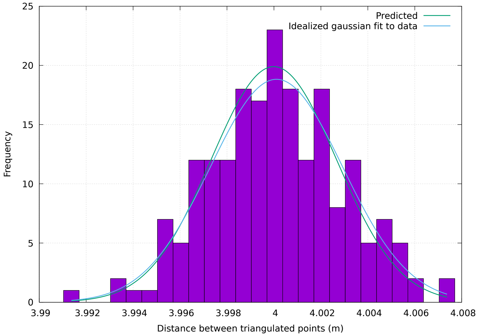
Distance between the two triangulated points: sample-stabilized
