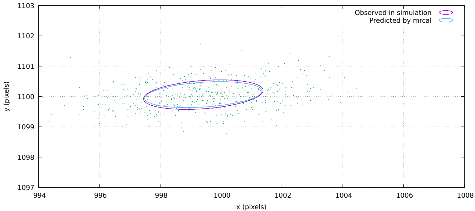
Surveyed calibration: distribution of point projections due to calibration-time noise
