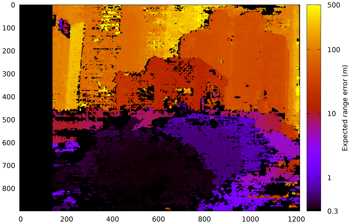
Expected range error assuming disparity error of 1.3 pixels
