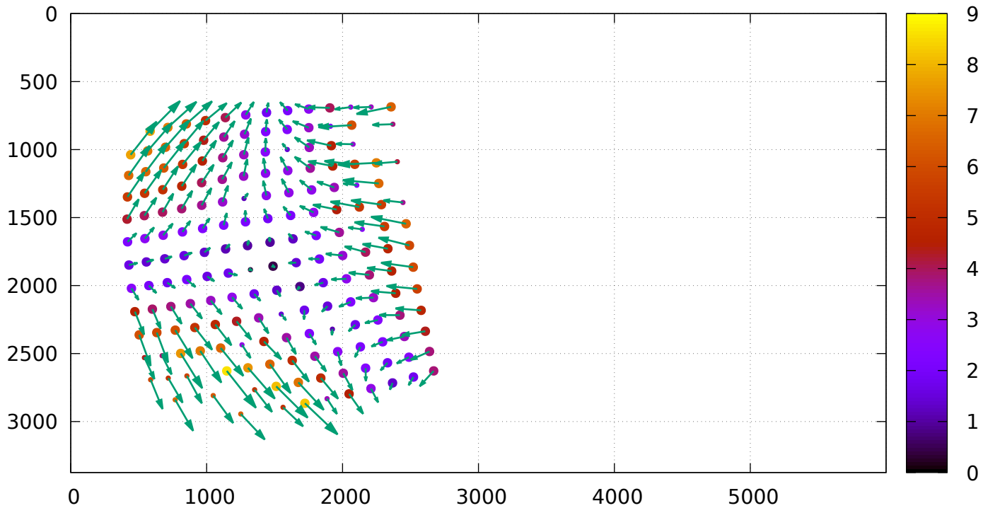
Residuals from a rolling shutter camera
