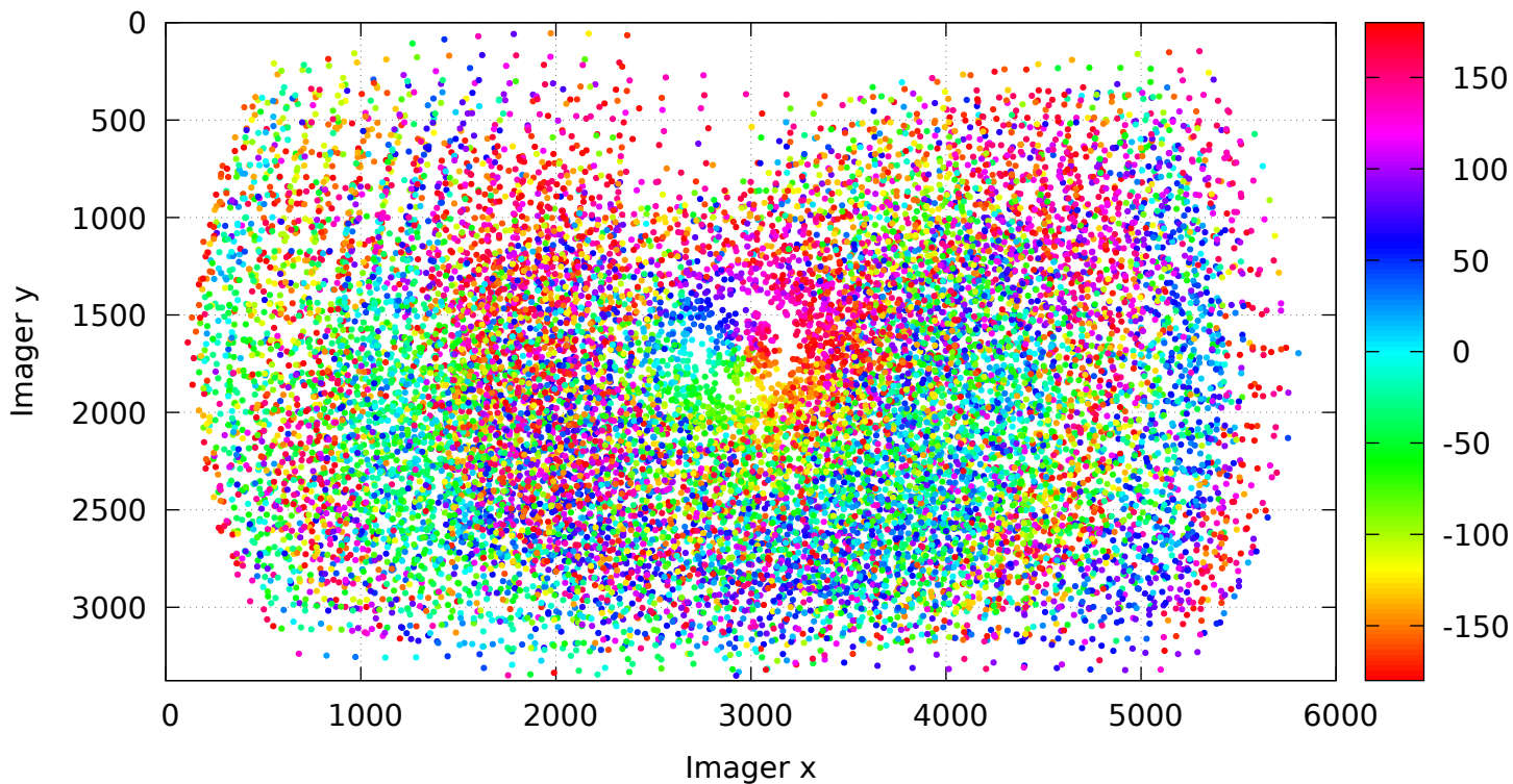
Fitted residuals. Directions shown as colors. Magnitudes ignored
