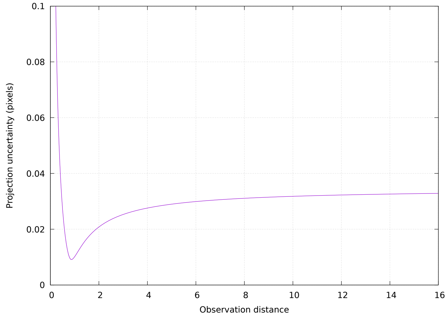
Projection uncertainty (in pixels) based on calibration input noise at q = center
