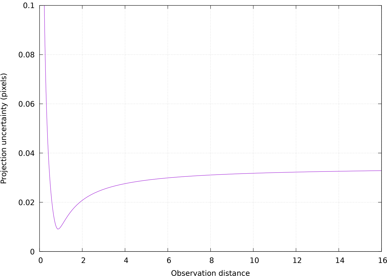
Projection uncertainty (in pixels) based on calibration input noise at q = \text{center}
