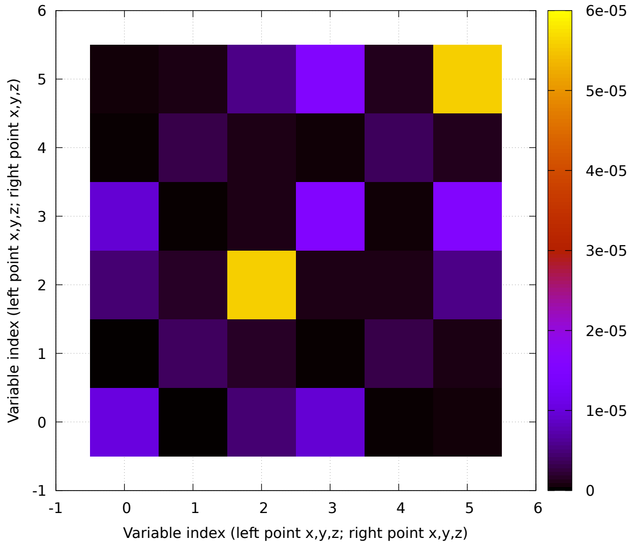
Abs(Covariance) of the [p0,p1] vector (m 2 ): sample
