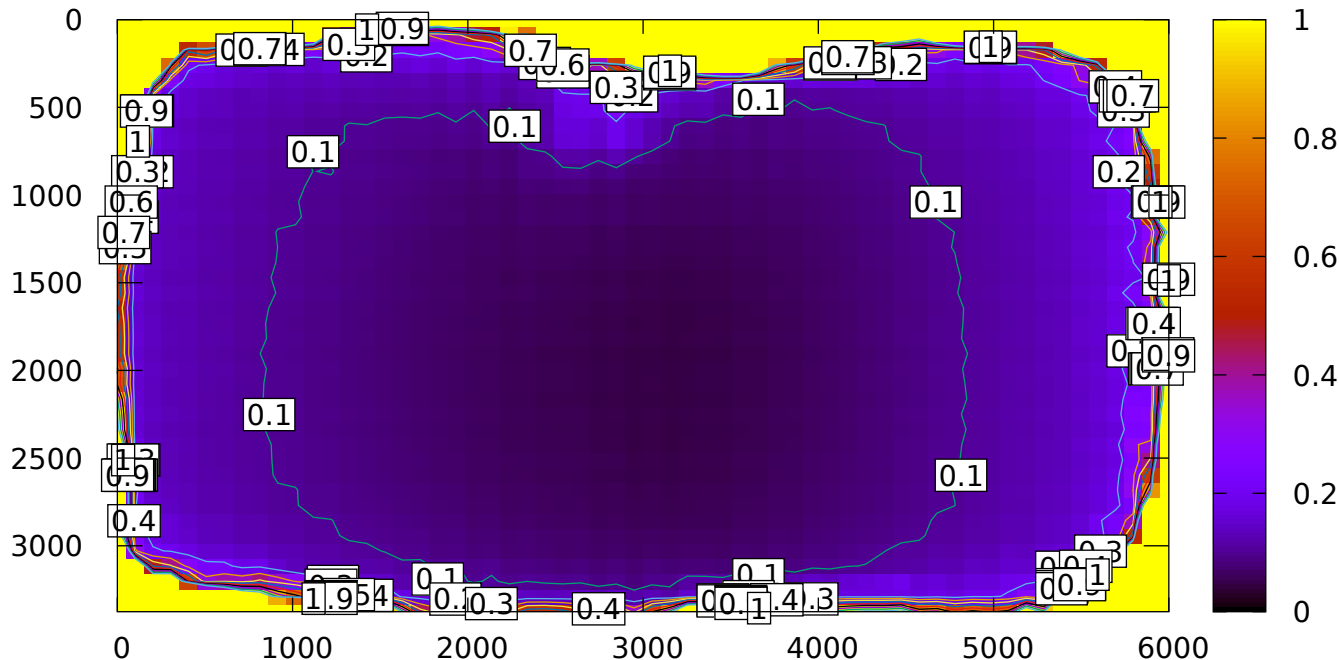
Projection uncertainty (in pixels) based on calibration input noise. Looking out to infinity
