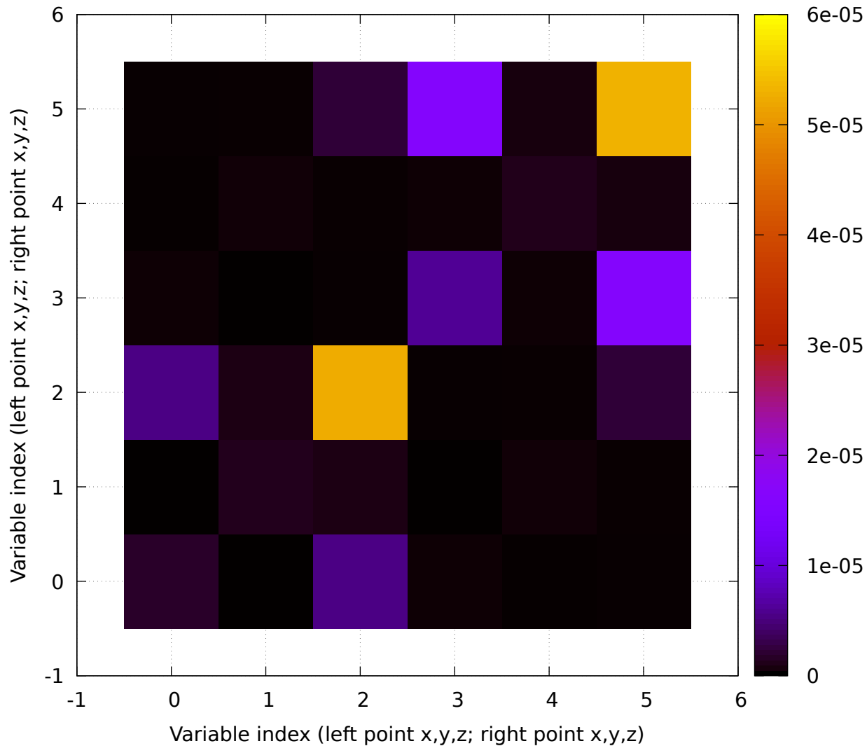
Abs(Covariance) of the [p0,p1] vector (m 2 ): sample-stabilized
