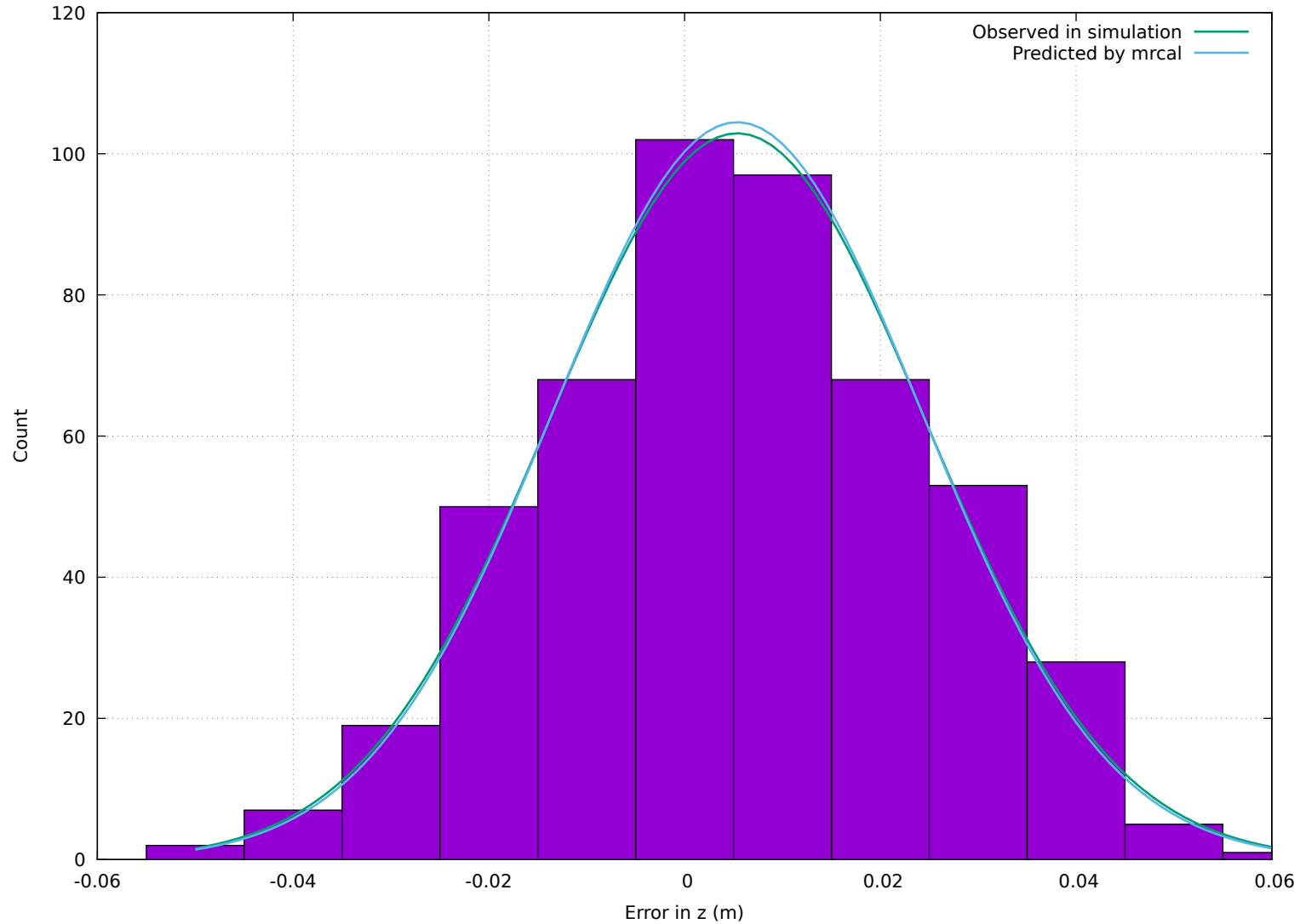
Surveyed calibration: distribution of error-in-z due to calibration-time noise
