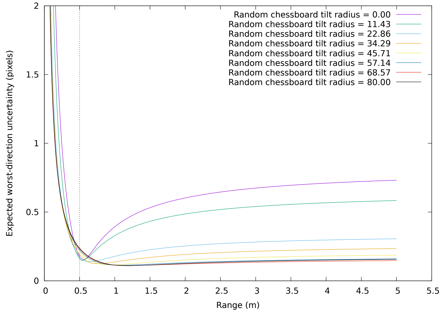
Scanning the board tilt. Have 1 cameras looking at 100 boards at 0.50m
