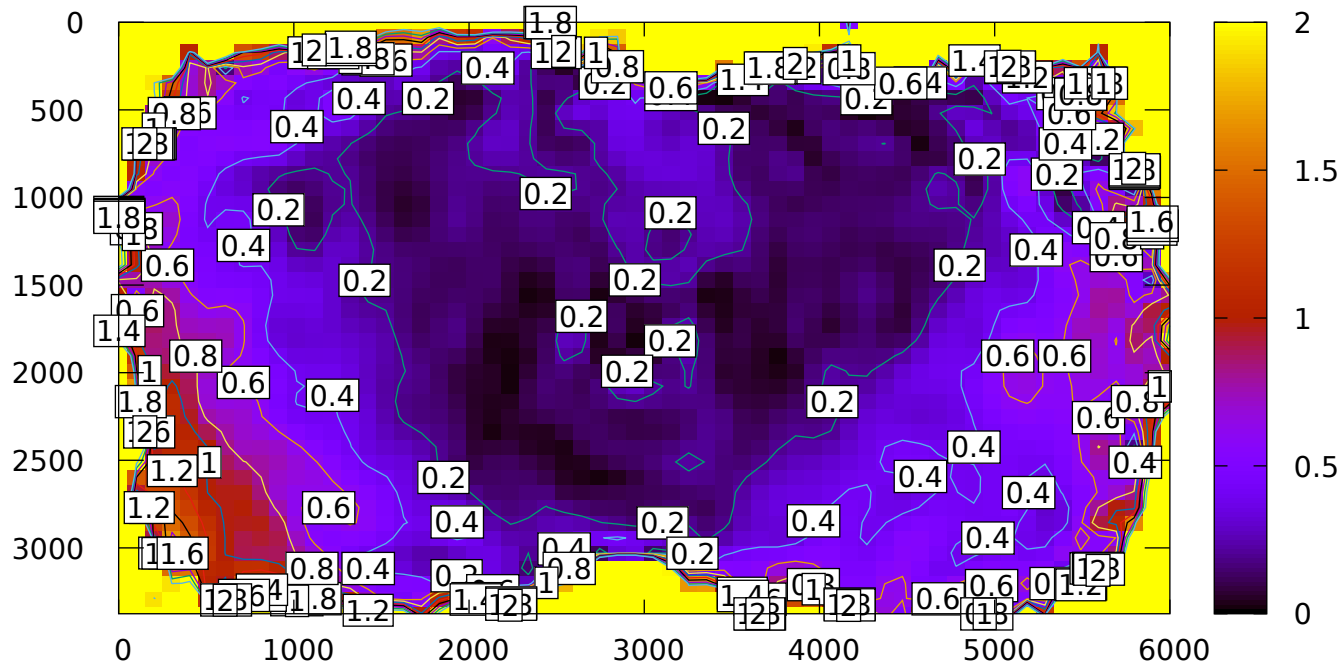
Cross-validation for LENSMODEL_SPLINED_STEREOGRAPHIC, noncentral
