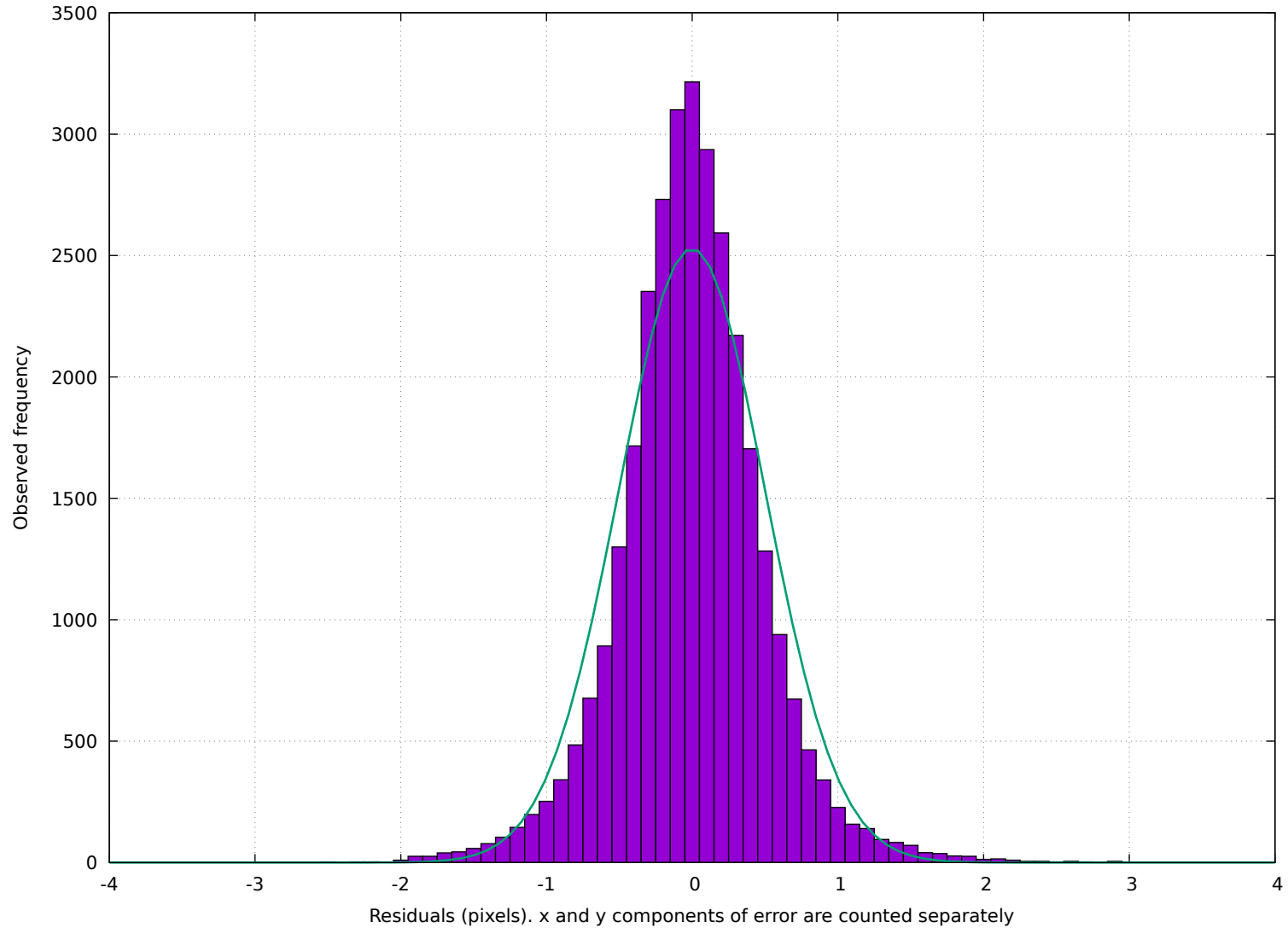
Observed and expected distribution of fitted residuals for all the cameras
