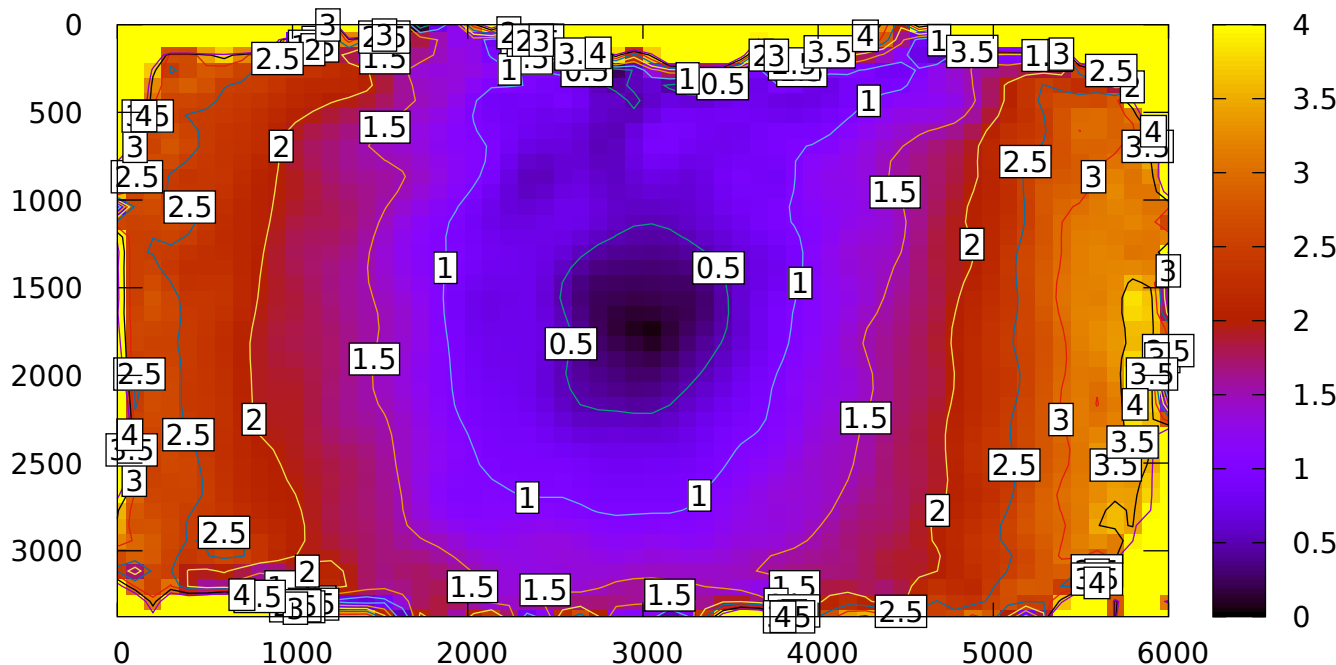
Projection error due to a dynamic chessboard shape error
